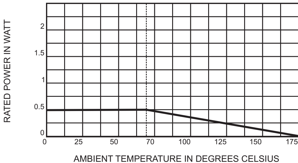
Derating Curve
